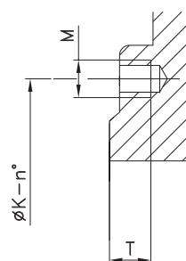
DN 10" - 14"
